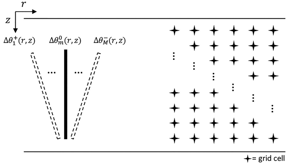
FIG. 1. Multiple tilt constraints (MTC) imposed on the vertical array. A positive angle ( \Delta\theta^+ ) is assigned to a counter-clockwise rotation in the source-receiver plane. The constraint matrix \mathbf{E} in Eq. (6) is composed of M replica vectors, \mathbf{e}_{\Delta\theta} , corresponding to various tilt angles between positive ( \Delta\theta^+ ) and negative ( \Delta\theta^- ) values with no array tilt ( \Delta\theta_m^0 = 0^\circ ) in the middle (thick line).
