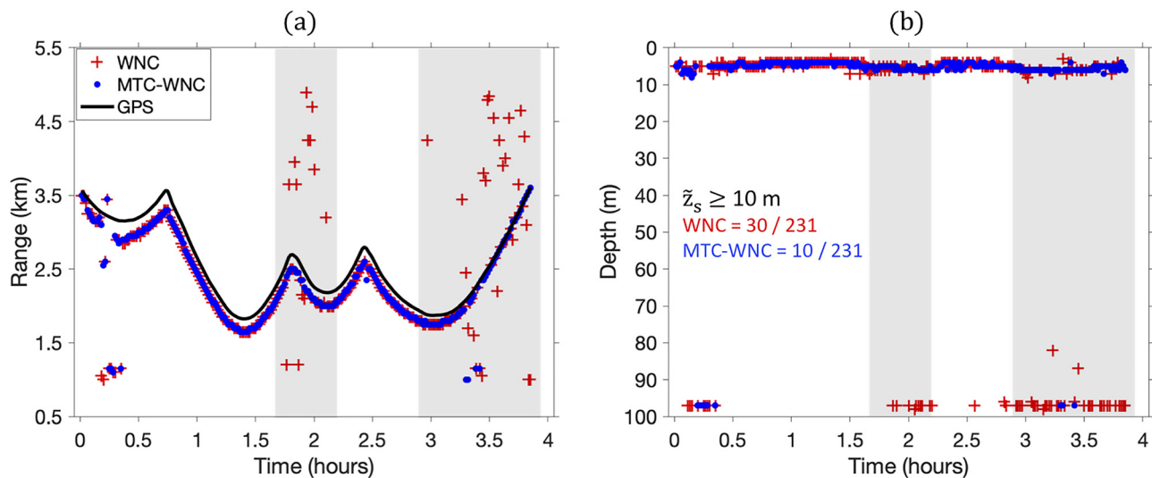
FIG. 6. (Color online) (a) Range estimate of the R/V Onnuri over the 4-h period, for the WNC (+) and MTC-WNC (•). The solid line indicates the ship GPS. (b) The corresponding depth estimate. The number of samples whose estimated depth is deeper than 10 m (i.e., bottom) is 10 out of 231 for the MTC-WNC, compared to 30 for the WNC. Note that most of the WNC errors occur in the shaded areas.
