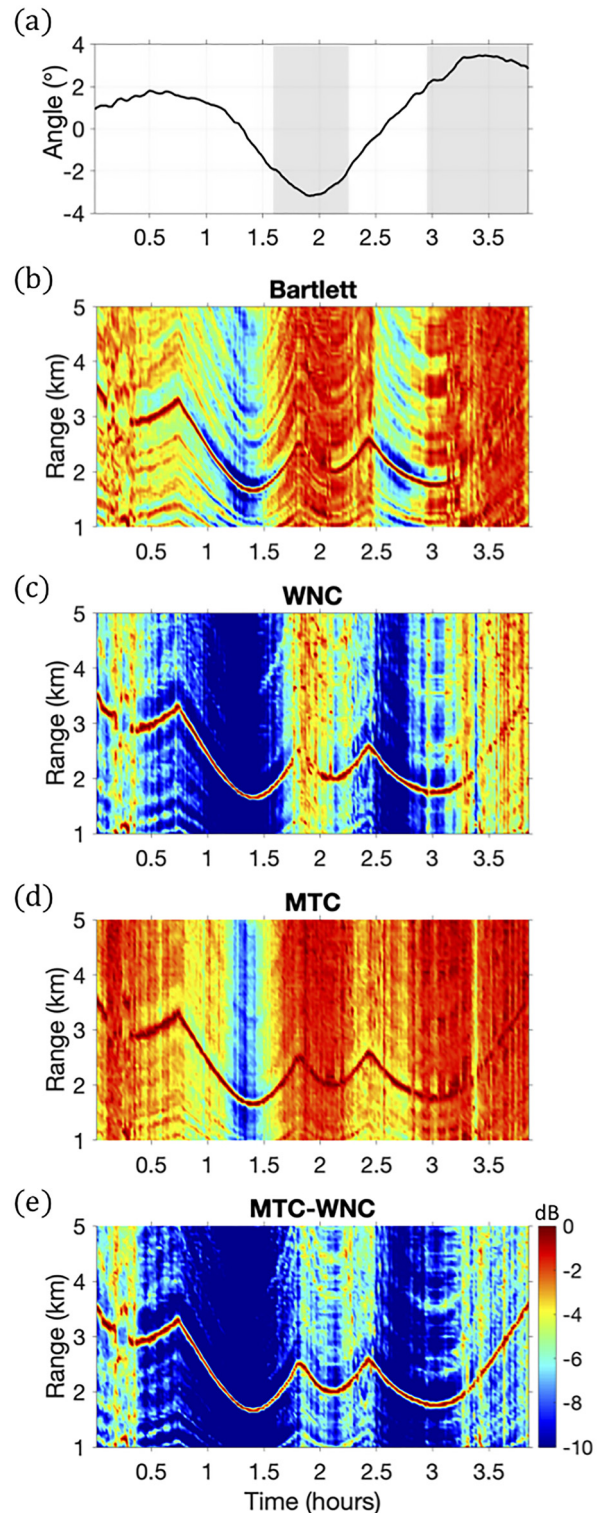
FIG. 5. (Color online) Range ambiguity at the estimated source depth [see Fig. 6(b)] for the entire 4-h period as depicted in Fig. 2(b), obtained by the (b) Bartlett, (c) WNC, (d) MTC, and (e) MTC-WNC. (a) Array tilt is separately estimated from the array invariant (Refs. 11, 15), and the shaded areas denote the period of large tilt angles, |\Delta\theta| \geq 2^\circ . The tracking performance of all processors except the MTC-WNC has deteriorated severely in those regions. However, (c) WNC has a significantly better sidelobe suppression performance than the other two (Bartlett and MTC) outside the regions, comparable to the MTC-WNC. (e) MTC-WNC consistently shows the best localization performance in the presence of even unknown environmental mismatch and a large array tilt with superior sidelobe control.
