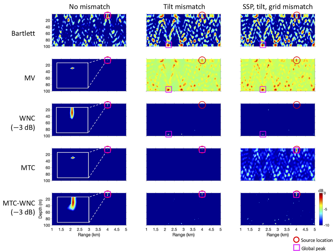
FIG. 3. (Color online) Simulated performance of various MFP processors for a 200-Hz source at range 4 km and depth 5 m: Bartlett, MV, WNC, MTC, and MTC-WNC. (Left column) No mismatch. (Middle) Array tilt mismatch ( \Delta\theta = +3^\circ ). (Right) Mismatch in SSP, array tilt ( \Delta\theta = +3^\circ ), and grid sampling [see Fig. 2(a)]. The region around the global peak for no mismatch (left column) is expanded. For MTC, a five-point tilt constraint ( M = 5 ) is applied at tilt angles, -4^\circ , -2^\circ , 0^\circ , +2^\circ , and +4^\circ . The circles and squares denote the true source position and the global peak, respectively. The MTC-WNC (bottom right) provides the most robust performance with a wider mainlobe and sidelobe suppression in the presence of environmental, array tilt, and sampling mismatch altogether. The dynamic range is 10 dB.
