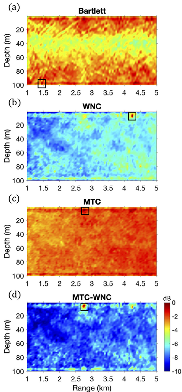
FIG. 4. (Color online) Ambiguity surfaces obtained with the R/V Onnuri at 2.7 km range depicted in Fig. 2(b) (green circle) for the (a) Bartlett, (b) WNC, (c) MTC, and (d) MTC-WNC. The array tilt was \Delta\theta = +3.3^\circ . The sample covariance matrix ( \hat{\mathbf{R}} ) was constructed from a 2-s window of the ship noise (200–500 Hz), and the power outputs were incoherently averaged across the bandwidth at 10 Hz intervals, yielding the global peaks ( \square ) either toward the surface or the bottom. Although (c) MTC has the global peak (2.7 km) close to the source range near the surface (5 m), the sidelobe/background levels are very high, within 2 dB from the mainlobe. Similar to Fig. 3 (right column), (d) MTC-WNC provides the best localization performance with a satisfactory sidelobe control in the presence of both unknown environmental mismatch and array tilt.
