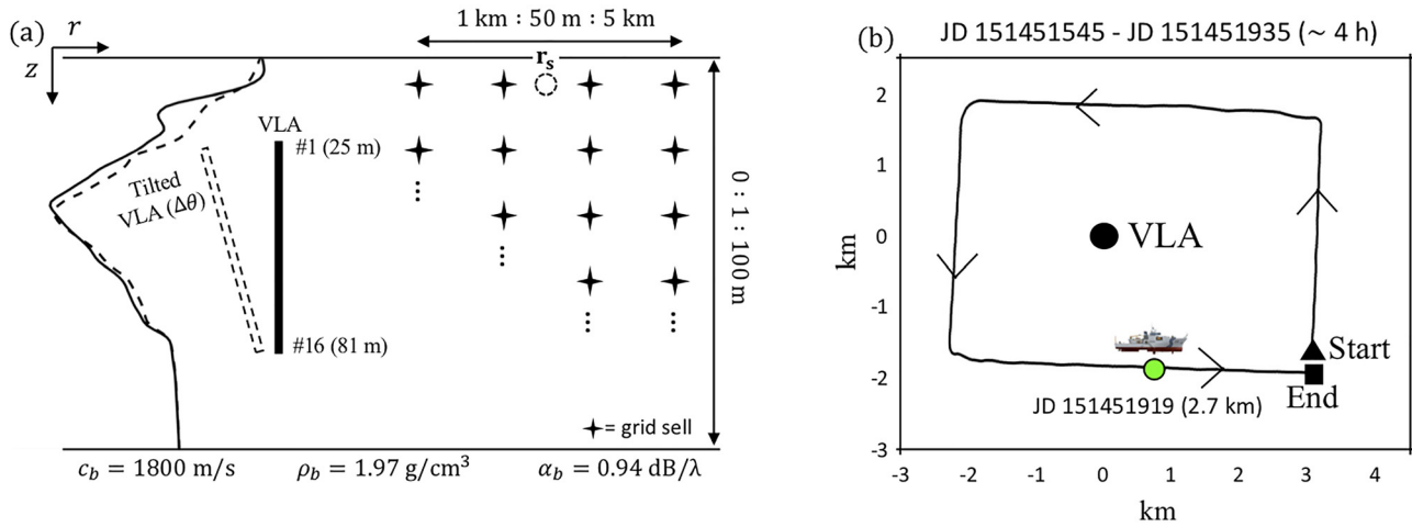
FIG. 2. (Color online) Schematic of the experiment conducted on JD 145 (May 25) during the source-tow run using the R/V Onnuri . (a) A 16-element, 56-m long, bottom-moored VLA in about 100-m deep water recorded the ship-radiated noise (200–500 Hz). The SSP (solid line) is an average of CTD profiles collected on JD 145, and the geo-acoustic parameters are shown in the bottom. For simulations in Sec. IV (see Fig. 3), three different types of mismatch are included (dashed): environment (SSP), system (array tilt), and grid sampling for a source at \mathbf{r}_s . (b) GPS ship track of the R/V Onnuri circling around the VLA at the origin counter-clockwise, mostly at a speed of 1.5 m/s for about a 4-h period (15:45–19:35 UTC). The green circle denotes the ship at 2.7 km range (JD 151451919) selected for evaluation of various MFP processors in Sec. V A (see Fig. 4).
